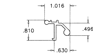
(13) SPRING LOADED LATCH
