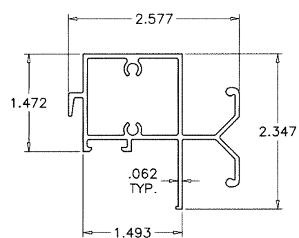
(5A) VENT TOP RAIL W/ HANDLE
