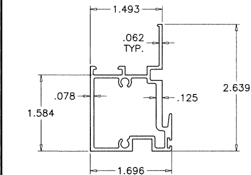
4 FIX. MEETING RAIL
