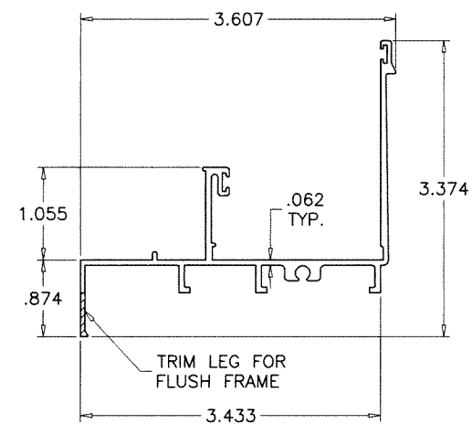
2 FRAME SILL
