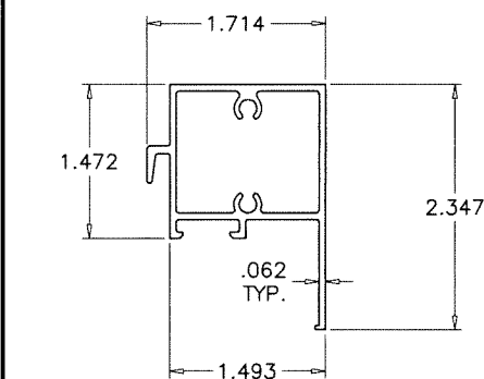
5 VENT TOP RAIL W/O HANDLE
