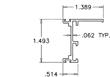
7 VENT SIDE RAIL
