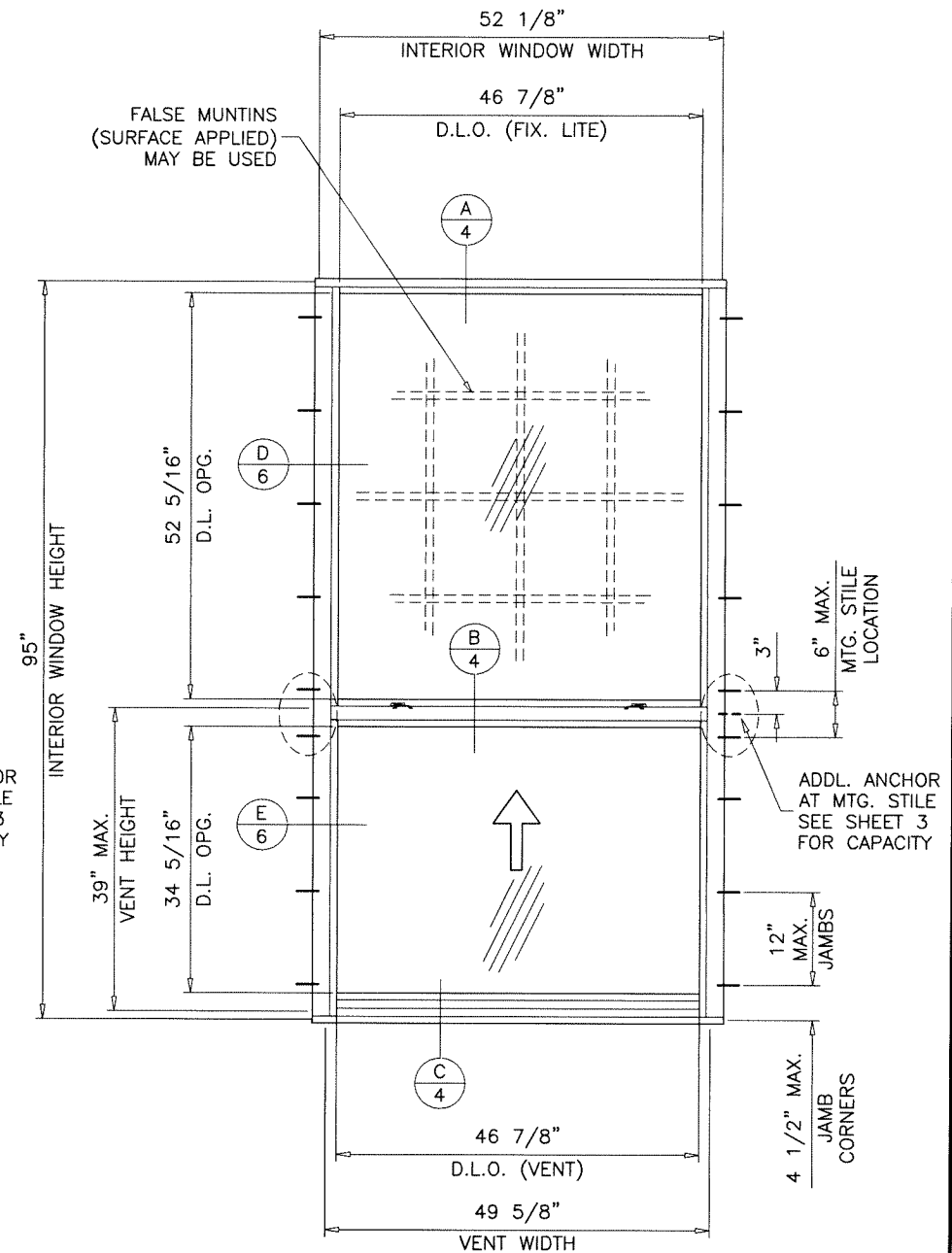
TYPICAL ELEVATION UNEQUAL LITES (ORIEL TYPE) TESTED UNIT
