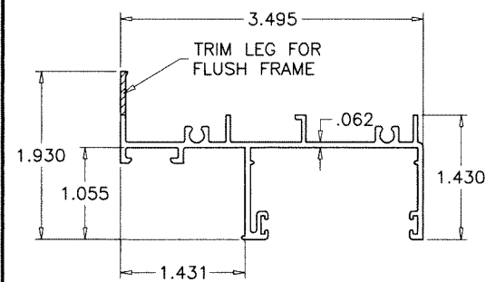
1 FRAME HEAD
